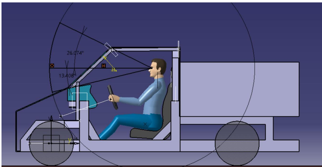
Figure 4 basic chassis design for goods van
